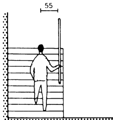
⑪ If stairs are straight and wide the distance of the line of walk to the handrails should be 55 cm
